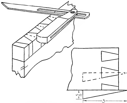
FIG. 268. MARKING DOVETAIL JOINT.
